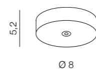
Ziko Base 1 AZ3408 (black) aluminium
